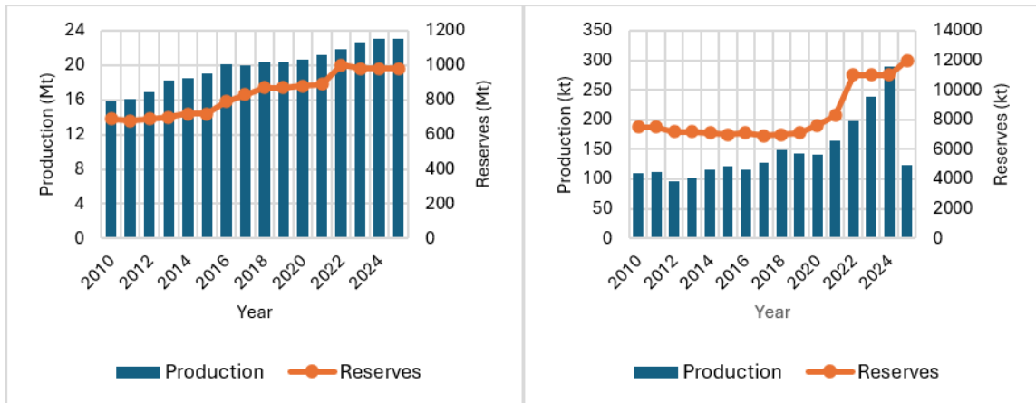
Figure 2 USGS (a) reported world copper production and reserves (b) reported world cobalt production and reserves (USGS, 2025a; USGS, 2025b)
